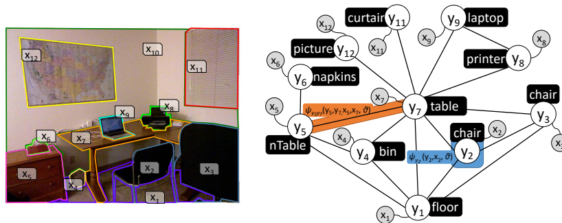
Figure 7. (Left) Scene from the NYUv2 dataset with segmented patches and their ids ( x_1 \dots x_{12} ). (Right) Conditional Random Field (CRF) graph built according to the patches in the NYUv2 scene (the node and relations of the wall, x_{10} , have been omitted for clarity). The orange area illustrates the scope of a pairwise factor modeling the relations between two objects, while the blue one stands for the scope of a unary factor classifying an object according to its features. Black boxes represent the expected results from a probabilistic inference process over such CRF.
