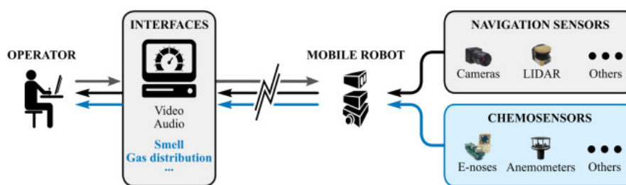
Figure 9. Diagram of a traditional teleoperation system (in black) and extended olfactory telerobotics (in blue). The latter requires equipping the mobile robot with additional sensors (e.g., an e-nose or an anemometer), and enhances the teleoperation user-interface to display this new sensory data.
