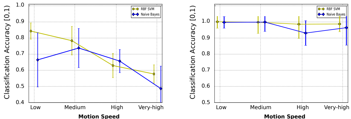
Figure 6. Average classification accuracy for different motion speeds using two classifiers (Naive Bayes and RBF SVM (Radial Basis Function for Supported Vector Machine)): (Left) classification accuracy when training the classifiers with static data samples; and (Right) results when the classifiers have been trained with data collected in motion.
