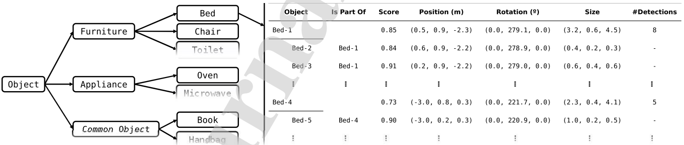
Figure 9: Excerpt of the content of an ontology after the inspection of the anto house by a mobile robot (instantiating a ViMantic client). The whole hierarchy of concepts was shown in Figure 3.
