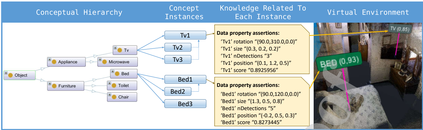
Figure 1: Example of a simple semantic map built by ViMantic . It includes a conceptual hierarchy modeling the properties of the elements appearing in the domain at hand as well as their relations, instances of those elements and their observed features, and a screenshot of the GUI designed to show part of that information to the user.
