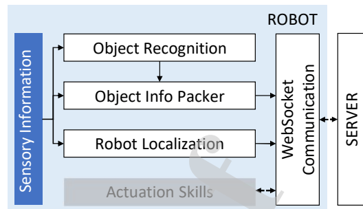
Figure 5: Overview of the proposed client side of the architecture showing its main components and their interconnections. White boxes are components, while the blue one represents sensors capturing data.
