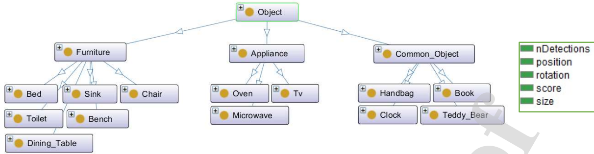
Figure 3: Left, excerpt of the proposed ontology exhibiting a hierarchy of concepts. Right, properties associated with instances of those concepts (inside a green box).
