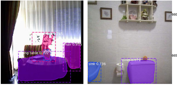
Figure 6: Object detections as reported by Detectron 2, part of the proposed recognition component. On the left, the CNN recognized a dining table with a confidence score of 0.702, a partially observed chair (0.935) and, even under bad lighting conditions, a potted plant (0.745). On the right, it detected a partially observed sink as well as a toilet with 0.736 and 0.979 confidence scores, respectively.
