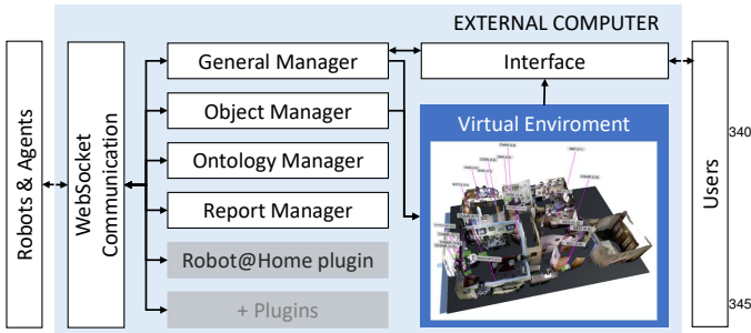
Figure 2: Overview of the proposed server side of the architecture showing its main components and their interconnections. The white boxes stand for components, the blue one represents the 3D virtual environment and the grey boxes are optional plugins that add extra functionalities.
