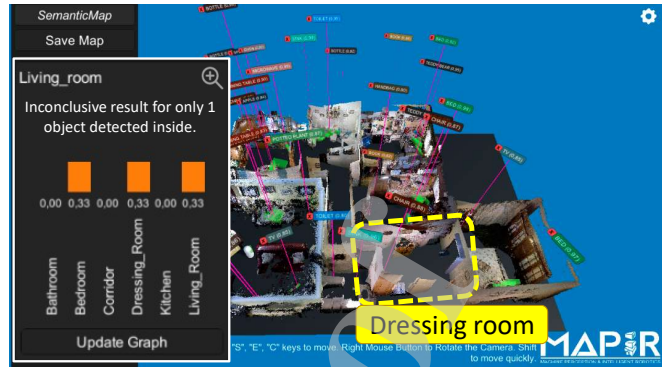
Figure 10: Use case of ViMantic where a plugin calculates the probability for the room to belong to a certain category (bathroom, kitchen, living room, etc.). This is done according to the objects that have been detected inside. In this case, the result obtained for the dressing room is inconclusive due to the lack of detected objects.
