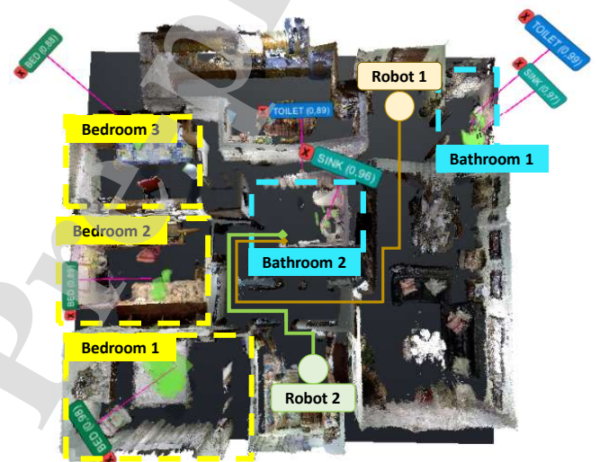
Figure 11: Example of a use case where a plugin decides which is the best suited robot for accomplishing the command “Check the tap in the bathroom near the bedrooms”. The discontinuous lines delimit the rooms, while colors represent their categories. The continuous lines show the path that each robot should follow to reach the target.
